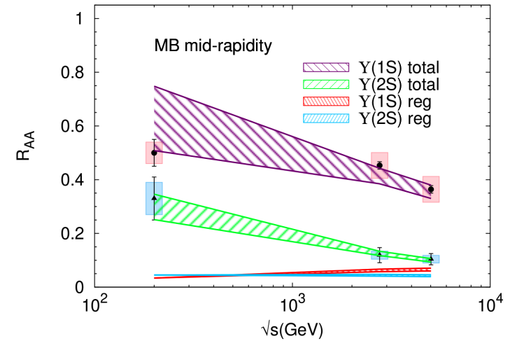
Figure 5.1: Excitation function of the nuclear modification factor for inclusive- J/\psi production in central Au-Au collisions at RHIC and in Pb-Pb collisions at the SPS and LHC (left panel), and for Y(1S) and Y(2S) production in minimum-bias collisions Au-Au and Pb-Pb collisions at RHIC and the LHC, respectively (right panel); TAMU transport model calculations are compared to data from the NA50, STAR, ALICE and CMS collaborations; figures are taken from Ref. [95].
