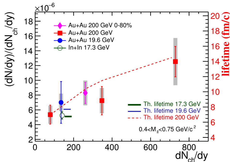
FIG. 6. (color online) Integrated yields of the normalized dilepton excesses for 0.4 < M_{ll} < 0.75 GeV/c 2 as a function of dN_{ch}/dy .
