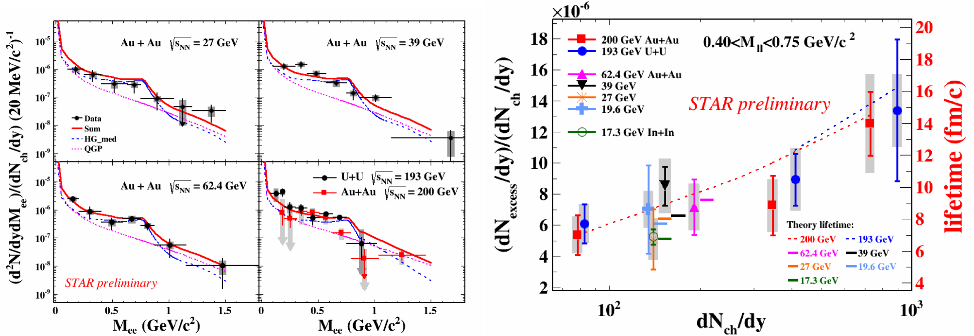
Fig. 5. (Left) Acceptance-corrected di-electron excess invariant-mass spectra normalized by dN_{ch}/dy in minimum-bias Au+Au collisions at \sqrt{s_{NN}} = 27, 39, 62.4 and 200 \text{ GeV} [26] and U+U collisions at \sqrt{s_{NN}} = 193 \text{ GeV} . Model calculations (red solid) with a broadened \rho spectral function which is the sum of QGP radiation contribution and in hadronic medium broadening [27][28] is shown. (Right) Integrated di-electron excess invariant-mass spectra ( 0.4 < M_{ll} < 0.75 \text{ GeV}/c^2 ) normalized by dN_{ch}/dy in different collision species and at different collision energies [26][29] compared to the theoretical calculations of the fireball lifetimes [27].
